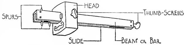
FIG. 33. MORTISE GAGE—SLIDE BAR.
